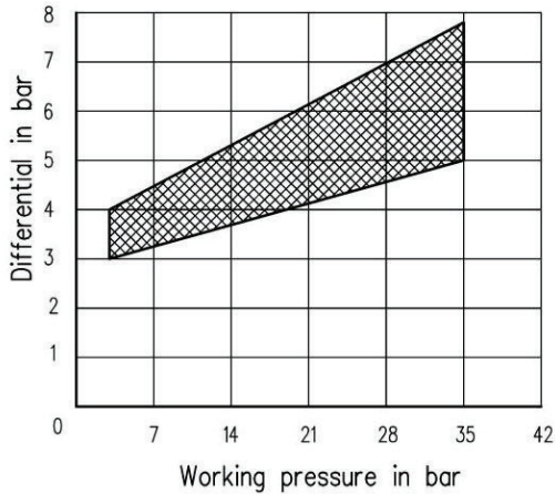
DIFFERENTIAL PRESSURE OF IPNB-160 PRESSURE SWITCH
