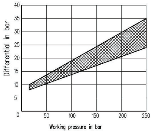
DIFFERENTIAL PRESSURE OF IPNB-630 PRESSURE SWITCH
