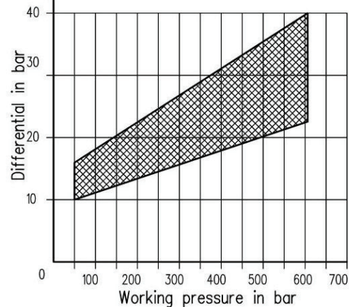
DIFFERENTIAL PRESSURE OF IPNB-630 PRESSURE SWITCH
