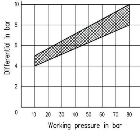
DIFFERENTIAL PRESSURE OF IPNB-250 PRESSURE SWITCH
