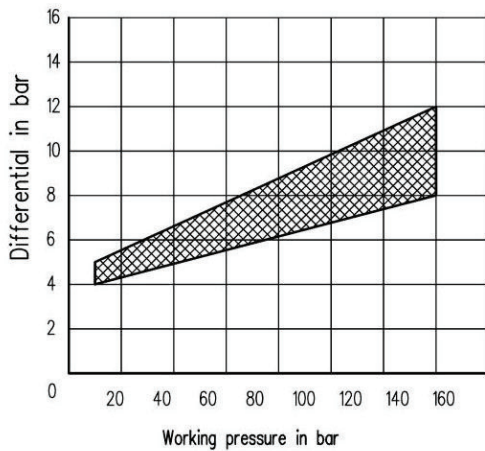
DIFFERENTIAL PRESSURE OF IPNB-350 PRESSURE SWITCH
